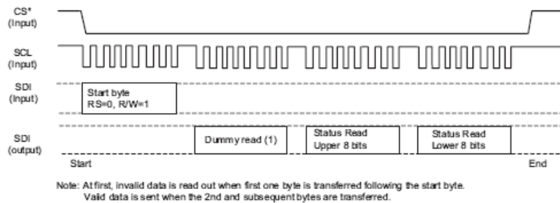
Figure 26: Serial interface data transfer timing
