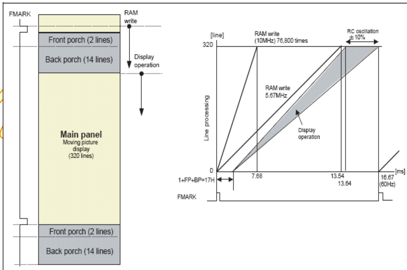
Figure 53: Write/Display Operation Timing
