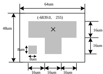
Alignment Marks-Left
