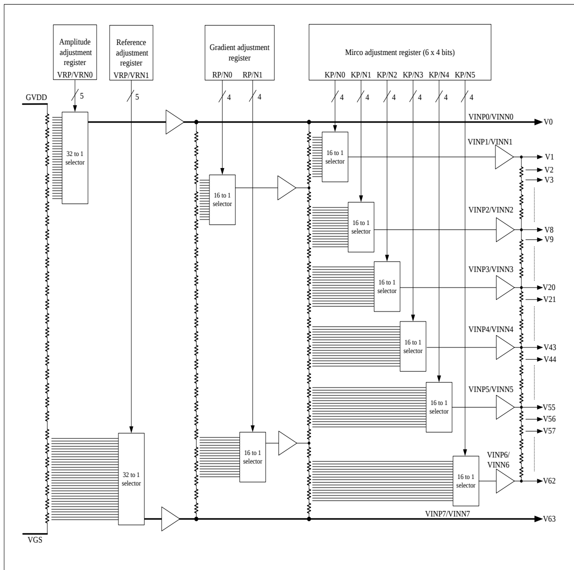
Figure36 Grayscale Voltage Generation
