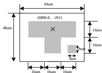
Alignment Mark-Right
