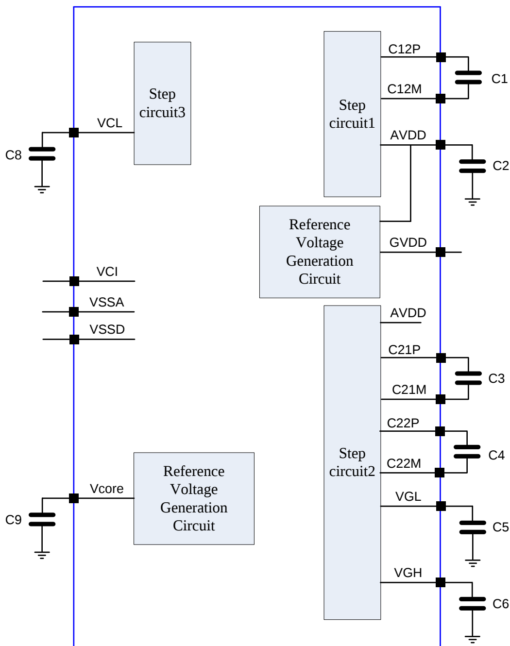
Block diagram of GC9312 power circuit
