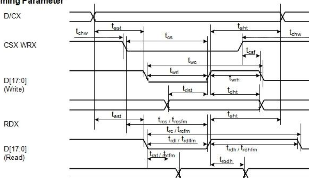
Figure 5.1 Parallel interface characteristics
