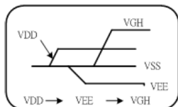
Power ON Sequence
