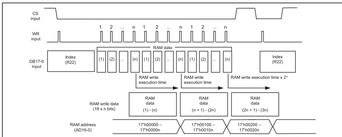
Figure 57 High speed RAM write operation timing relationship
