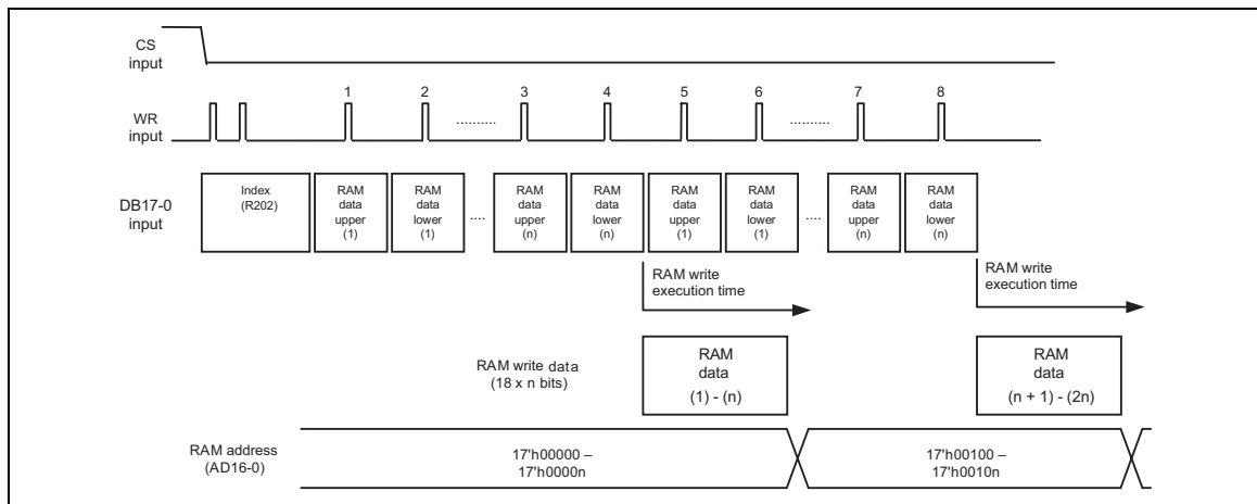
Figure 58 High speed RAM write operation via 9-bit interface
