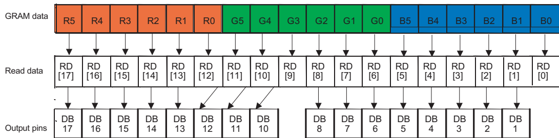
Figure 26 RAM data write/read (16-bit interface)
