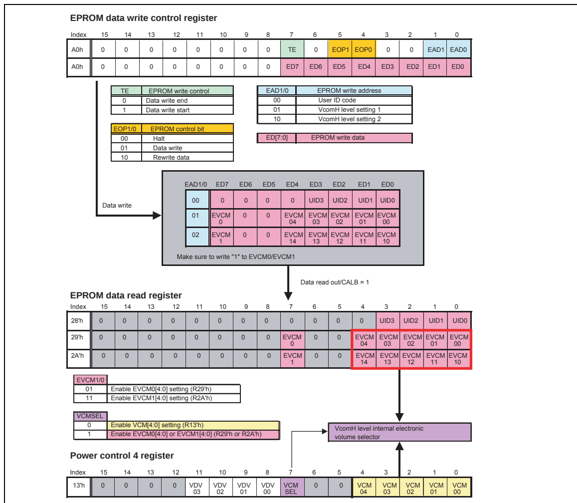
Figure 84 EPROM system configuration
