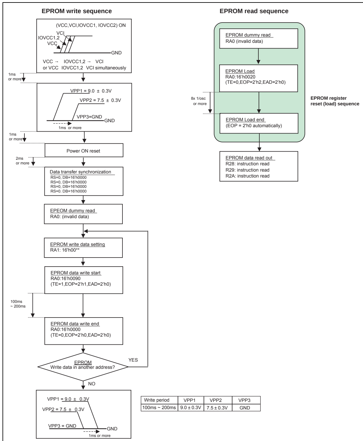
Figure 85 EPROM write sequence
