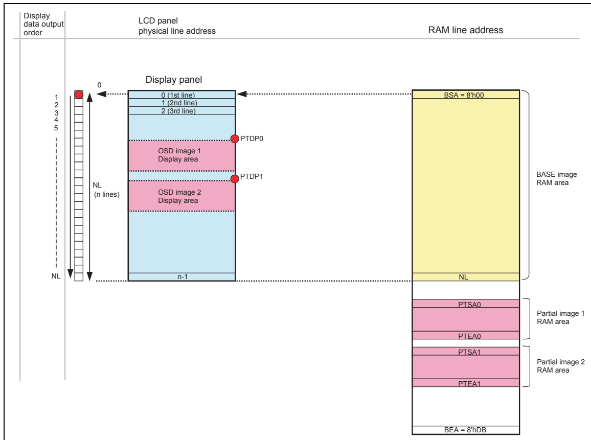
Figure 53 Display RAM address and panel display position
