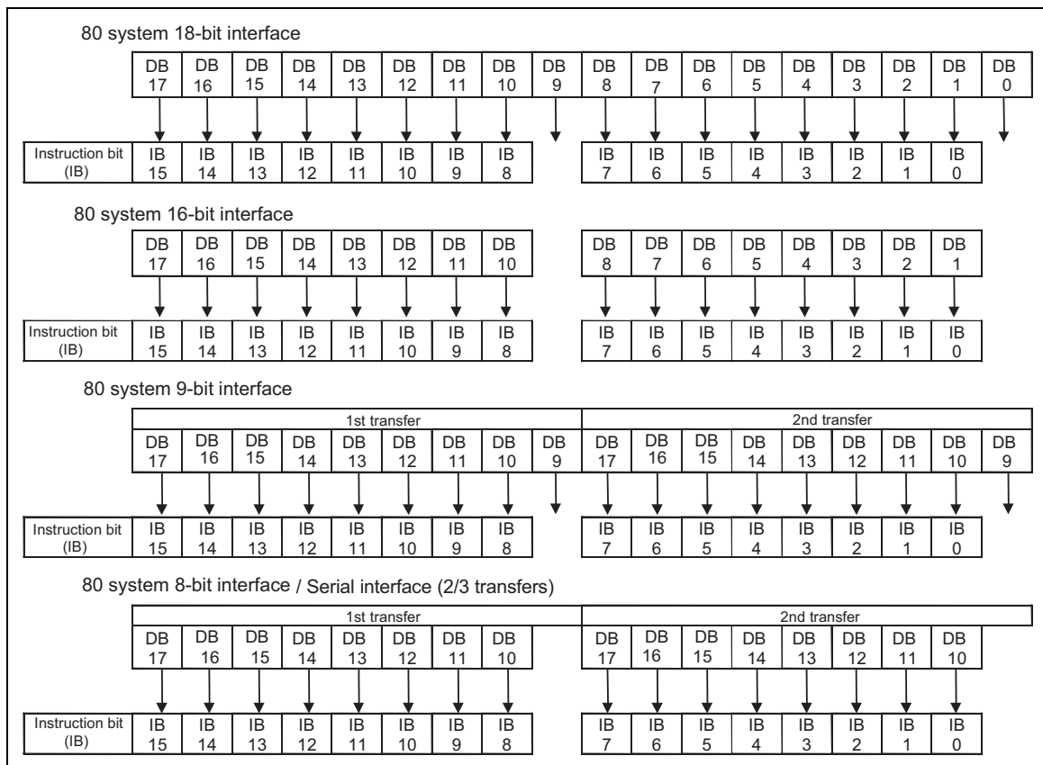
Figure 10 Instruction format
