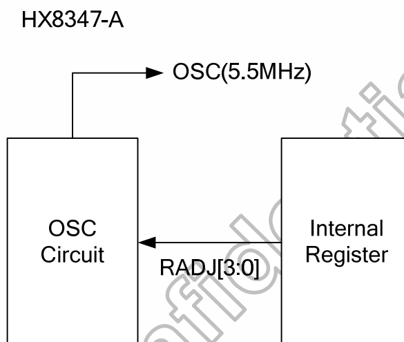
Figure 5. 41 Oscillation Circuit
